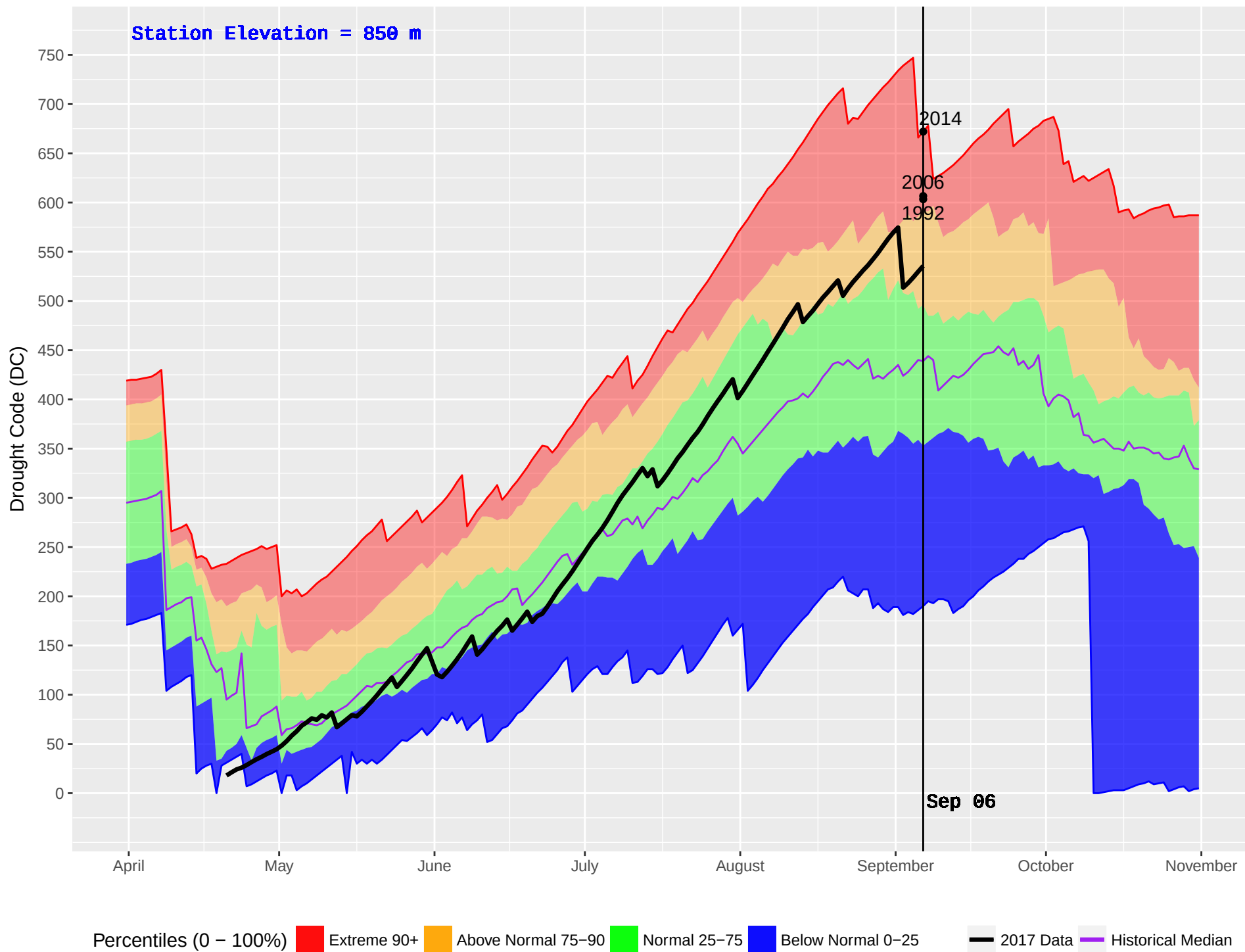
NORTH CHILCO (159) : Historical (1972–2016) and Current (2017) Noon Drought Code (DC)
